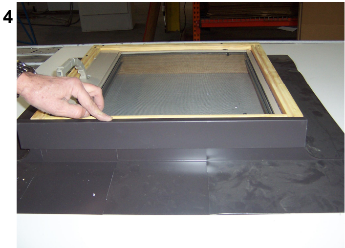
Remove rubber gasket and staples
