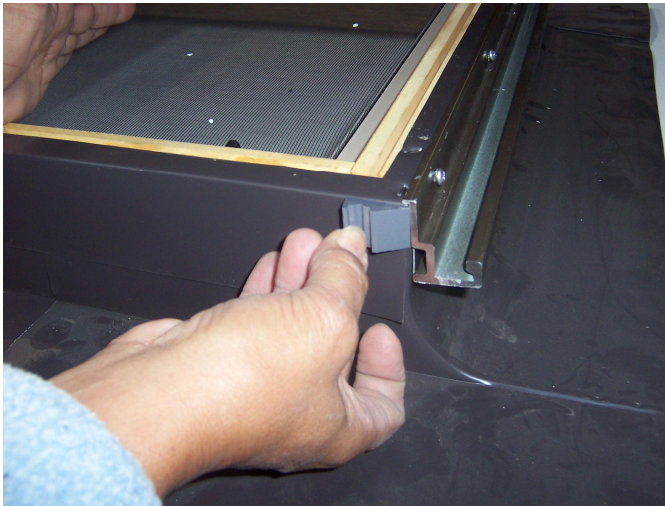
Install small guides on rear left & right corners
