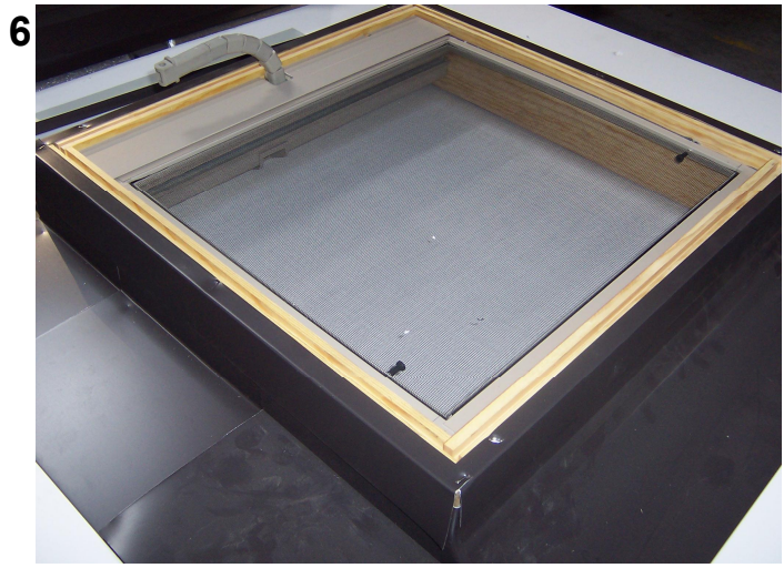
Image shows Counter Flashing Installed on all four sides.
