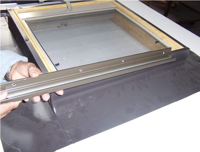
Install hinge on rear of curb
