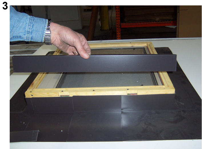
Install Counter Flashing on all Four Sides.
